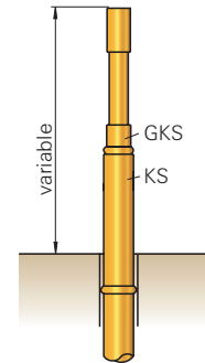
Example for usage of KS-112 ... G8 (with Press-ring)
